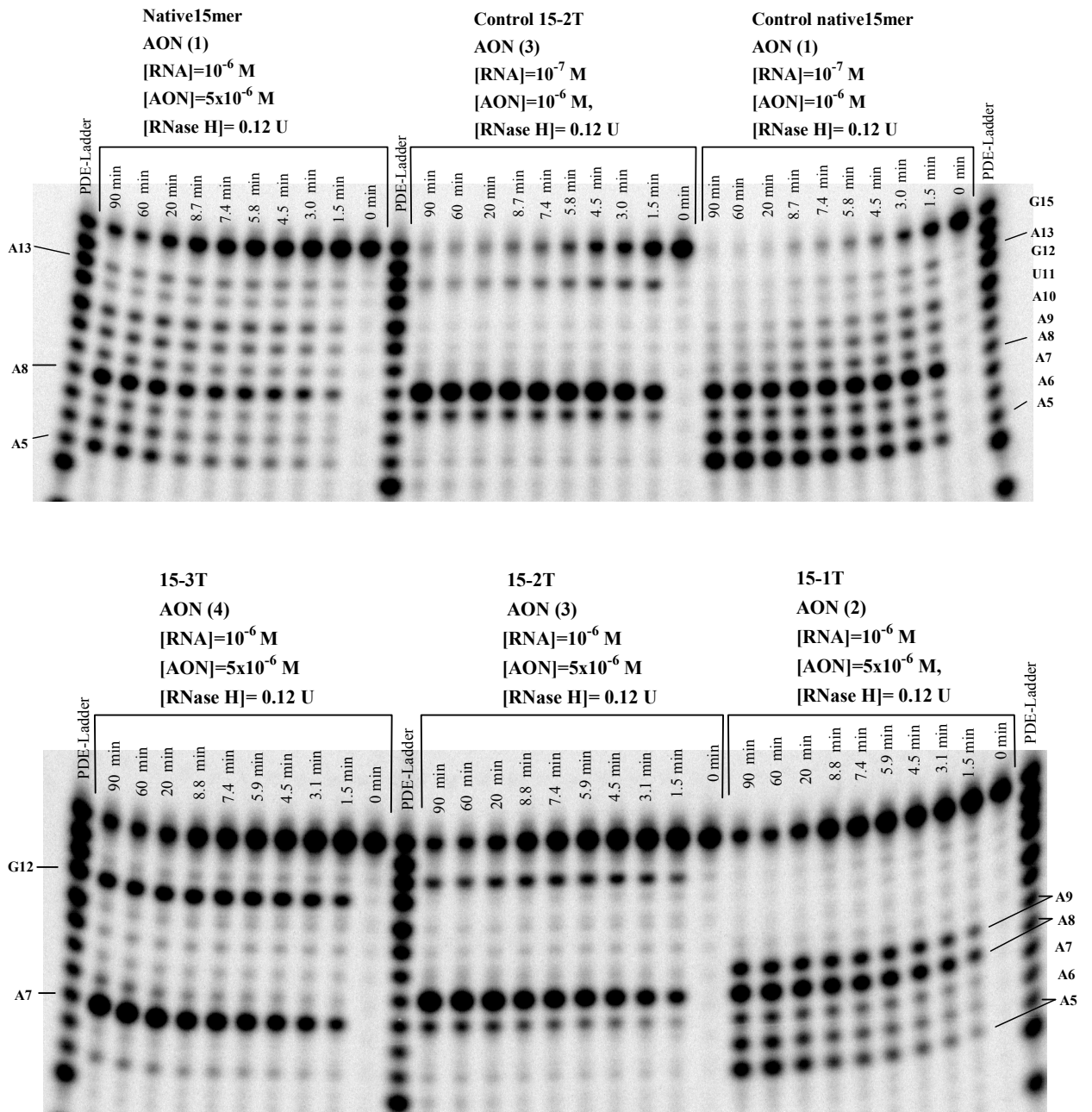
Figure S13. Autoradiograms of 20% denaturing PAGE, showing the cleavage kinetics of 5'- 32 P-labelled target RNA ( 14 ) by RNase H1 in the native AON ( 1 )/RNA ( 14 ) and the single, double and triple oxetane T modified AON ( 2-4 )/RNA ( 14 ) hybrid duplexes. The kinetics of the control native 15mer AON ( 1 ) and double T AON ( 3 ) with 1 \mu M and RNA ( 14 ) with 0.1 \mu M concentration, used for the calibration of the exact RNase H concentration, are also shown. PDE-Ladder: snake venom PDE ladder. Conditions of cleavage reaction: RNA (0.1 or 1 \mu M) and AONs (1 or 5 \mu M) in buffer, containing 20 mM Tris-HCl (pH 8.0), 20 mM KCl, 10 mM MgCl 2 and 0.1 mM DTT at 21 °C, 0.12 U of RNase H. Total reaction volume is 30 \mu l. (See Materials and Methods section for full experimental details.)
